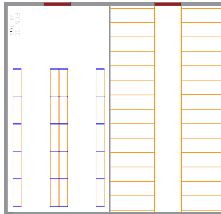
C5, 1,000sqm, store non critical DG parts
